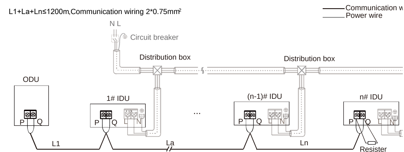
Figure 3-8.6: P Q communication wiring configuration – IDUs uniform power supplied
