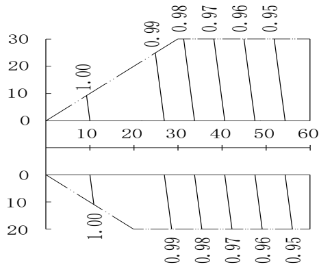
Figure 2-8.3: 100 model rate of change in cooling capacity
