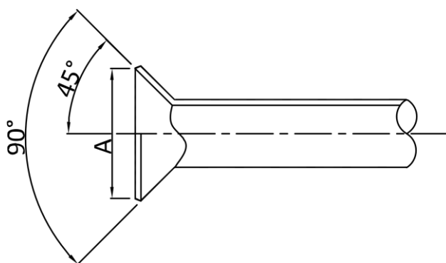
Figure 3-4.2: Flared opening
