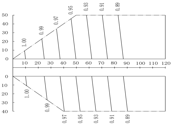
Figure 2-8.7: 140 model rate of change in cooling capacity
