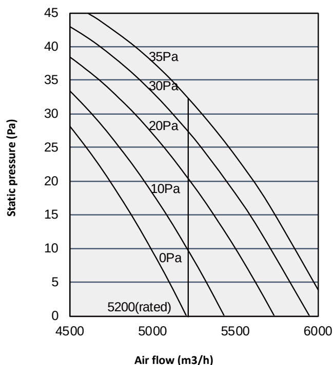
Figure 3-2.5: 80/100 model units fan performance
