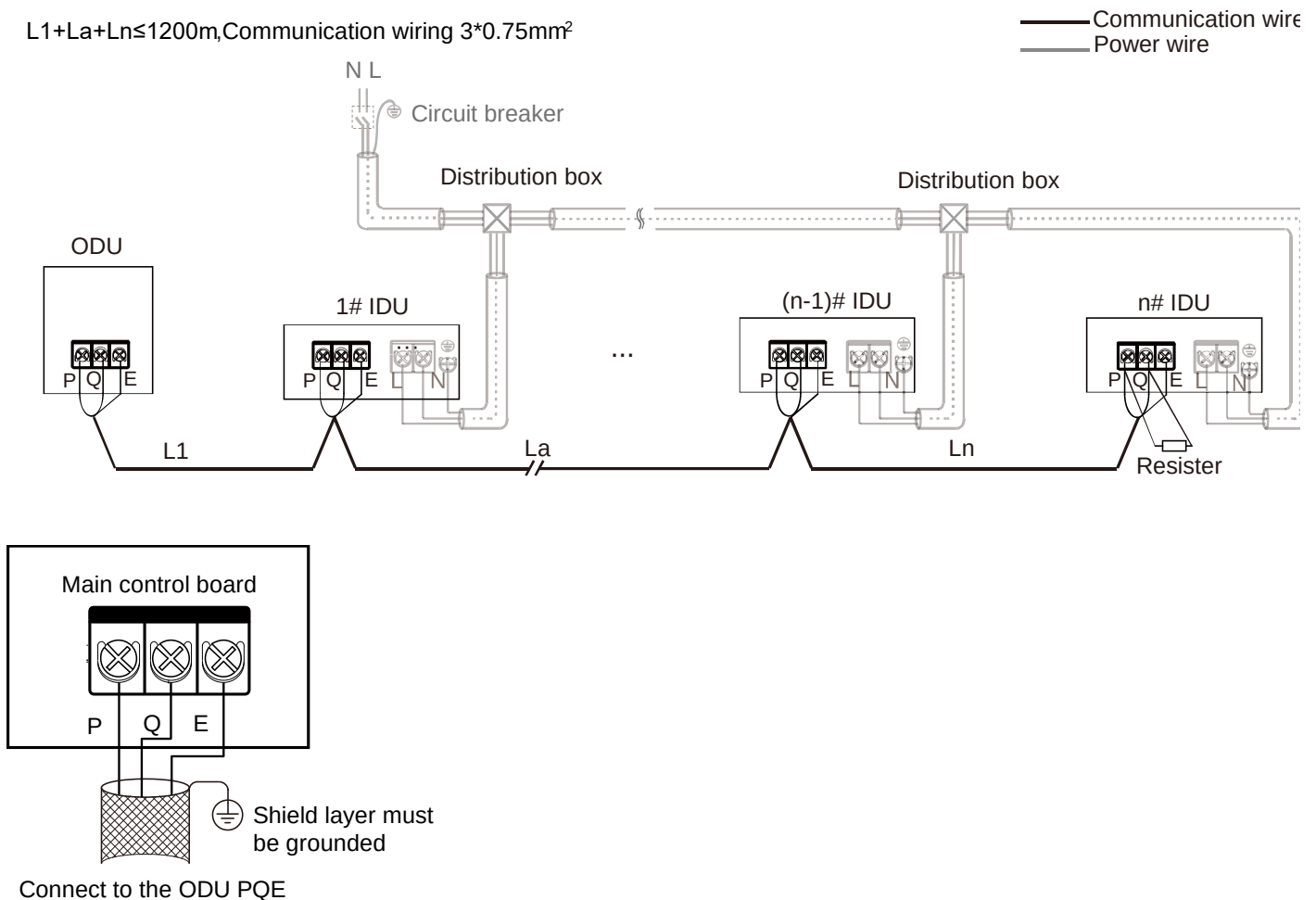
Figure 3-8.5: P Q E communication wiring configuration – IDUs uniform power supplied
