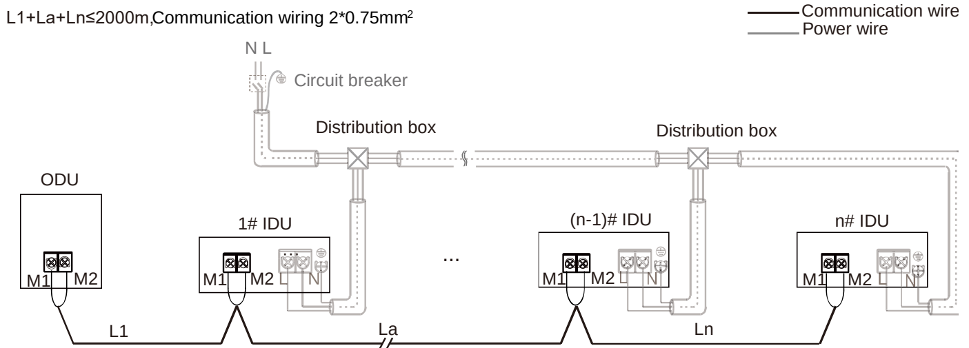
Figure 3-8.7: M1 M2 communication wiring configuration – IDUs uniform power supplied
