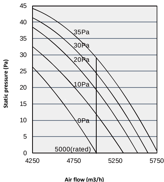
Figure 3-2.6: 120/140/160 model units fan performance
