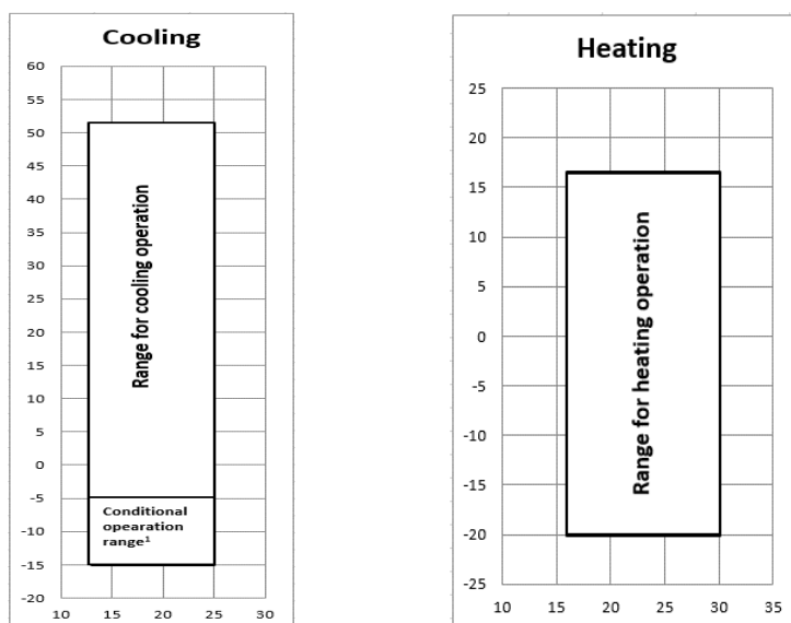
Figure 2-9.1: Operating limits
